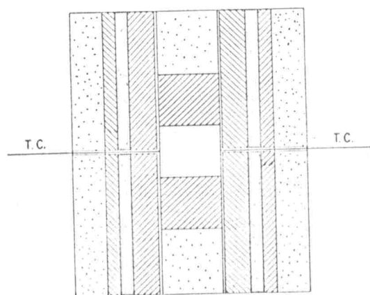
Fig. 1. High-pressure chamber. Light stippling is massive pyrophyllite (lava), crosshatched areas are alumina, and the heavy stippling is the graphite heater. Sample at the center is enclosed in Pt foil. Thermocouple wires pass through the cell in protection tubing (not shown). ( \times 50 .)
